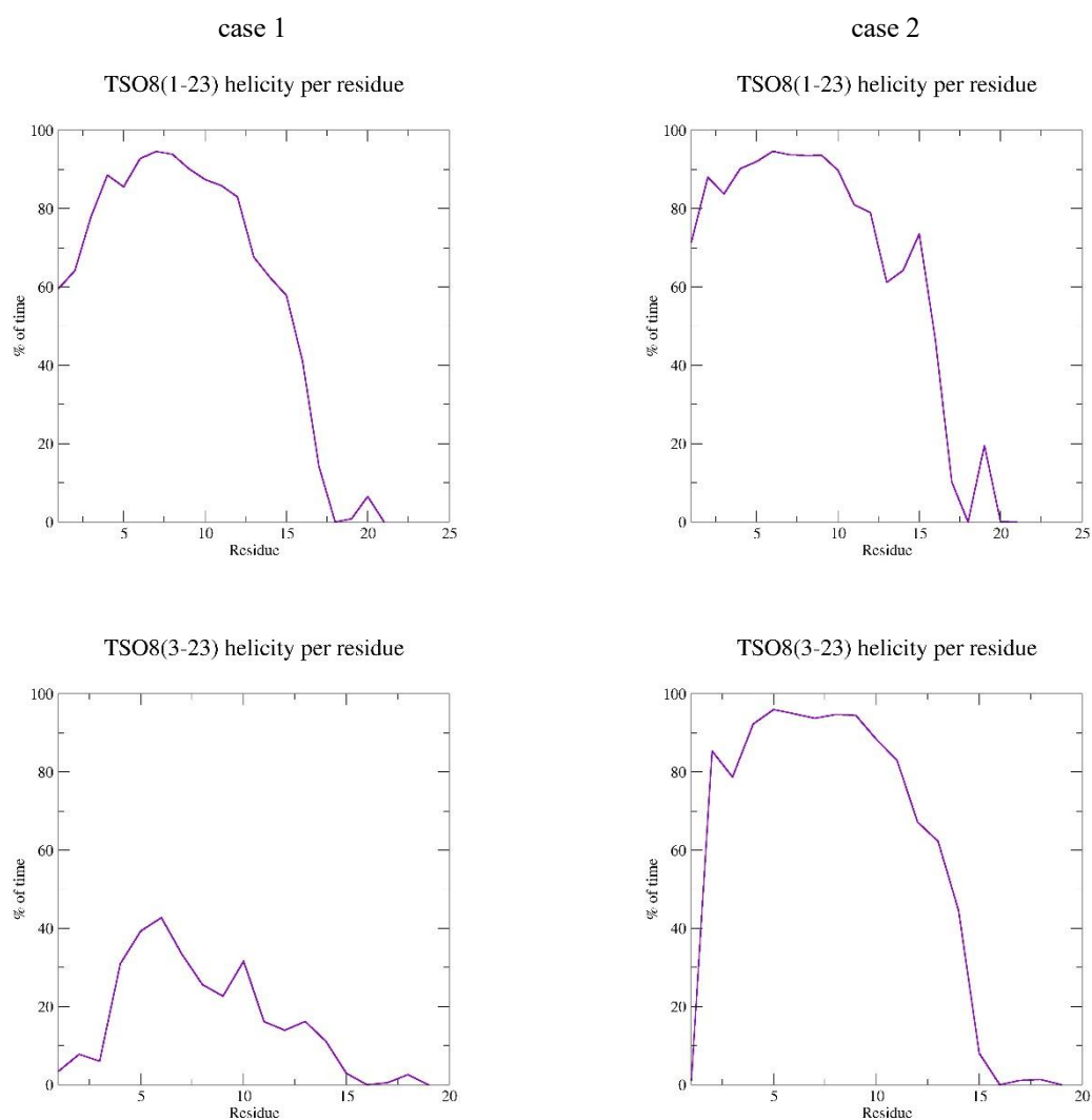
Figure 47 Helicity per residue calculated for TSO8(1-23) and TSO8(3-23) during the 500 ns simulation in water (left) and 1.0 \mu s simulation with the membrane (right)
