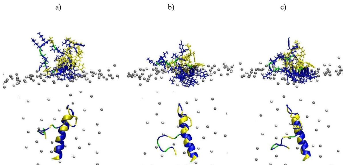
Figure 14 Snapshots from 1.5 \mu s long simulation of TSO8_lin near the POPE:POPG membrane. Side (top) and top (bottom) view of peptide states at times a) t=100 ns, b) t= 500 ns and c) t=1.5 \mu s. Amino acids are coloured according to their hydrophobicity (polar – blue, hydrophobic – yellow, glycine - green). Membrane is represented only by P atoms of the upper leaflet (POPE – silver, POPG - white). Water molecules and ions are not shown for clarity.
