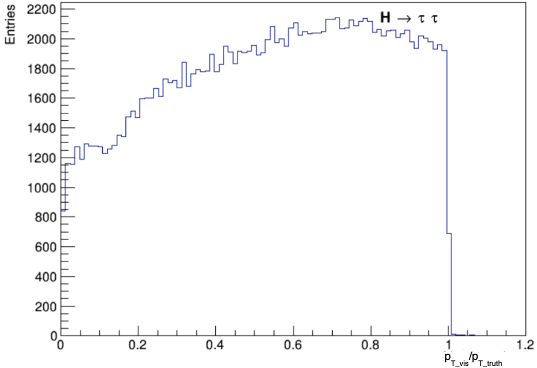
Figure 34: Ratio of transverse momentum of \tau_{vis} and \tau_{truth}
