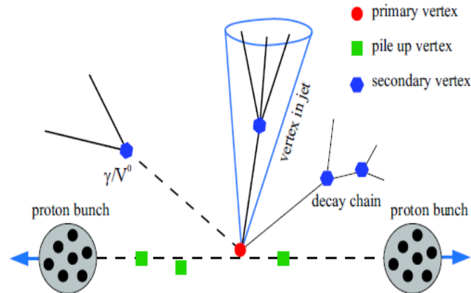
Figure 16: Aftermath of a proton-proton collision with multiple vertices. Taken from [12]
