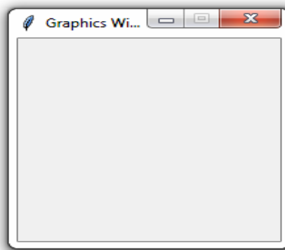
Slika 5.1. Graphics Win
