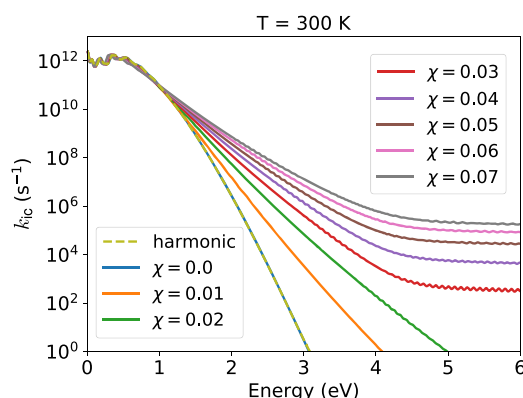
FIG. 5. CIMMC in cyhex. Internal conversion rates from an anharmonic AS model for different degrees of anharmonicity \chi . The dashed line shows the rate obtained with FCclasses3 for the AS model, which should be identical to the \chi = 0.0 case.
