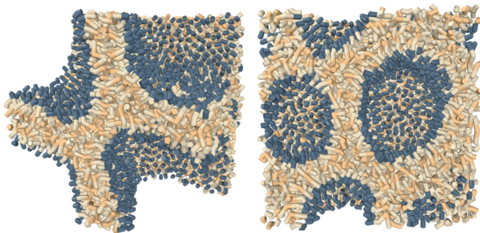
Figure 12: Visualized trajectories; network on the left, sponge on the right.
