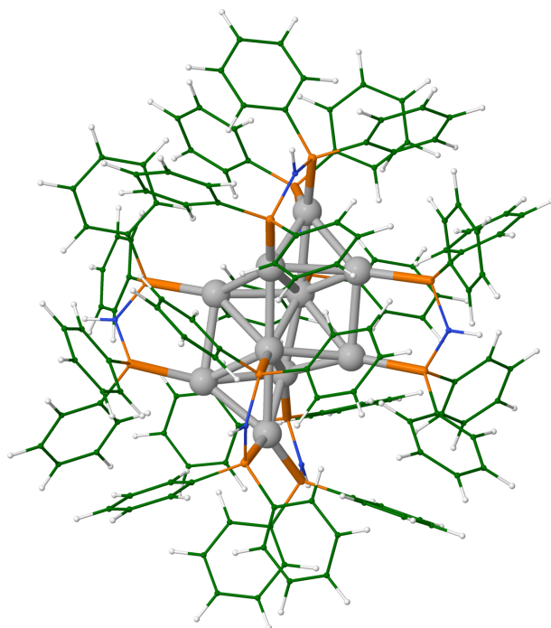
Figure S17: Fully optimized structure of [Ag_{10}(dppa)_6]^{2+} . Color legend: Ag (silver); P (orange); N (blue); H (white) and C (green).
