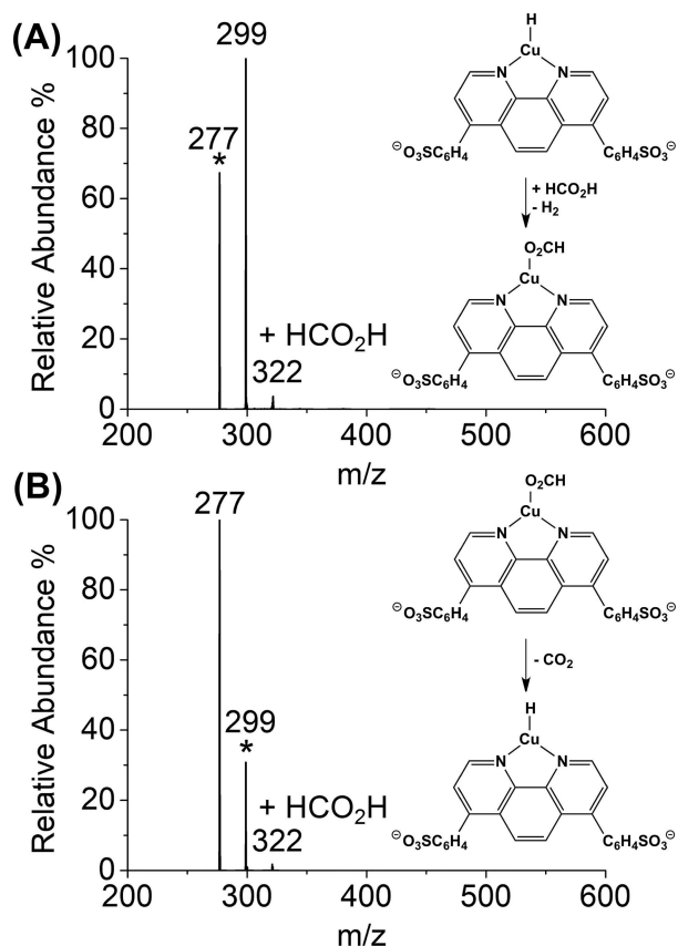
Figure 1. LTQ mass spectra obtained for the MS n CID (or IMR) experiments of: (a) IMR of [(phen*) 63 Cu(H)] 2- ( m/z 277), 1 d , with formic acid; (b) CID of [(phen*) 63 Cu(O 2 CH)] 2- ( m/z 299), 2 d . An activation time of 30 ms was used for the CID experiments and 500 ms for the IMR experiments. A * represents the mass-selected precursor ion.
