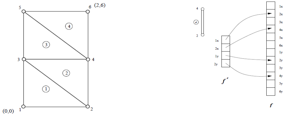
Figure A.1: A simple finite element mesh of triangular elements and an example of an element force vector \mathbf{f}^e scattered into a global force vector f
