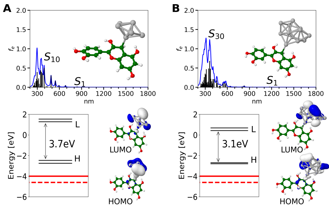
Figure S3: TDDFT calculated absorption spectra for the: A) (cyanidin-Ag 6 ) - , B) (cyanidin-Ag 12 ) - employing CAM-B3LYP/def2-SVP method. Structures have been optimized at PBE/def2-SVP level of theory.
