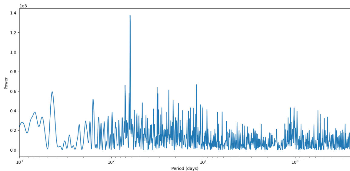
Figure 13 HD 3651 periodogram
