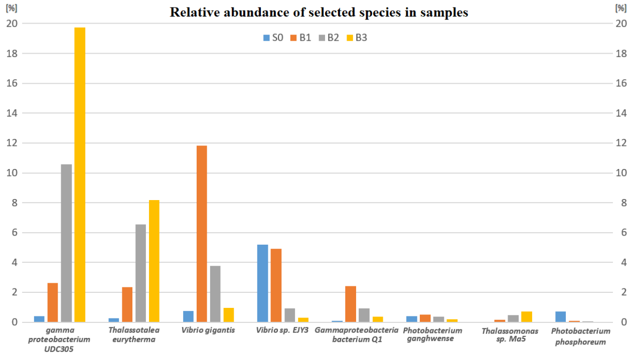
Figure 37. Relative abundance of pioneer bacterial species in seawater (S0) and during the first three days of biofilm formation on the surface of immersed slides (B1, B2 and B3).
