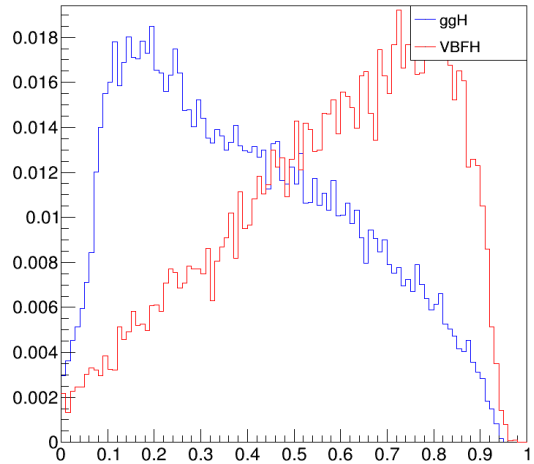
D_VBF1j for 350 GeV
